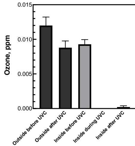
Fig. 11. Graph showing that during decontamination cycles, the ozone levels are below the limit of detection of the sensor in the horizontal cabinet.
